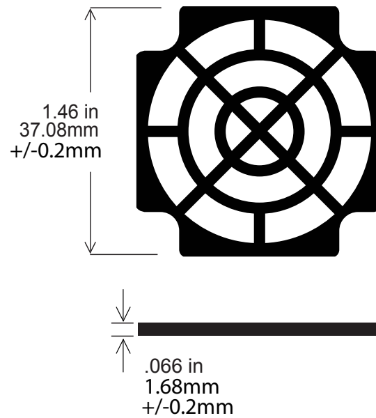
Retainer
